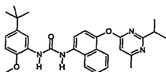
1-(5-tert-Butyl-2-methoxy-phenyl)-3-[4-(2-isopropyl-6-methyl-pyrimidin-4-yloxy)-naphthalen-1-yl]-urea;
